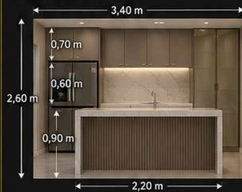
VISTA FRONTAL
